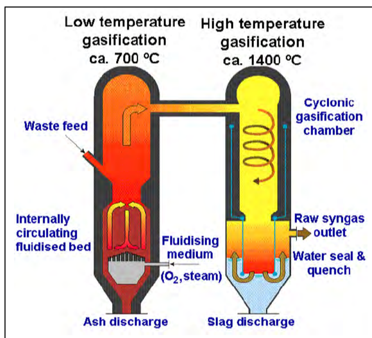
Figure 2.17: Fluidised bed gasifier with high temperature slugging furnace
